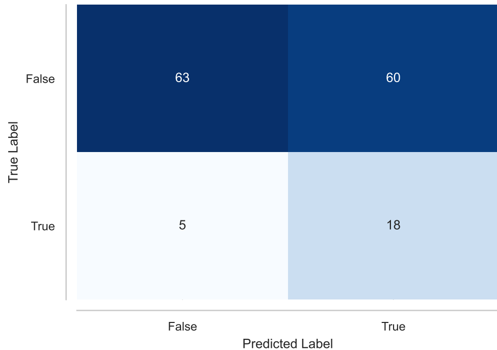
Confusion Matrix - RF
